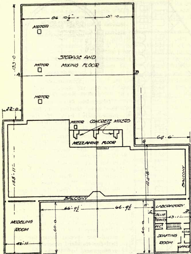
FIG. 124—SECOND FLOOR PLAN, PLANT NO. 10
